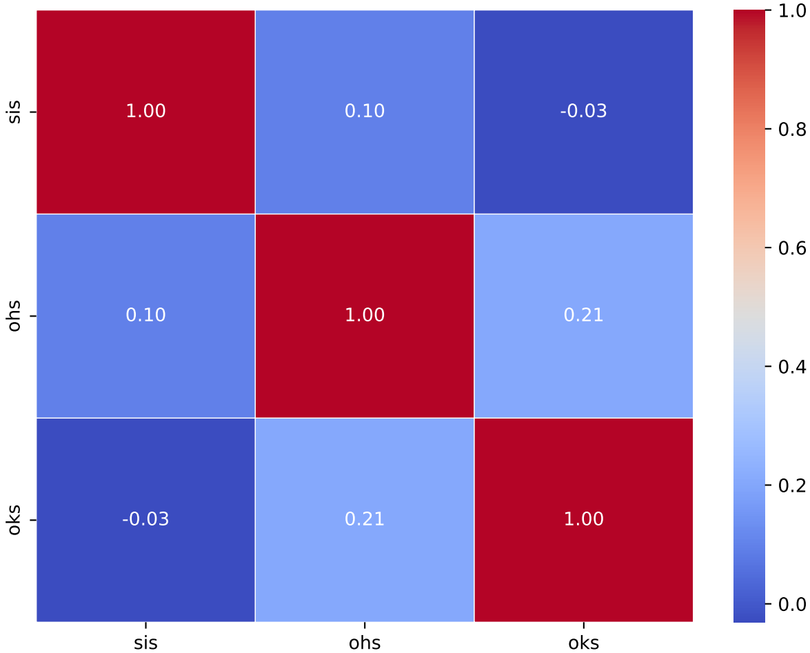
Kendall Correlation Matrix
